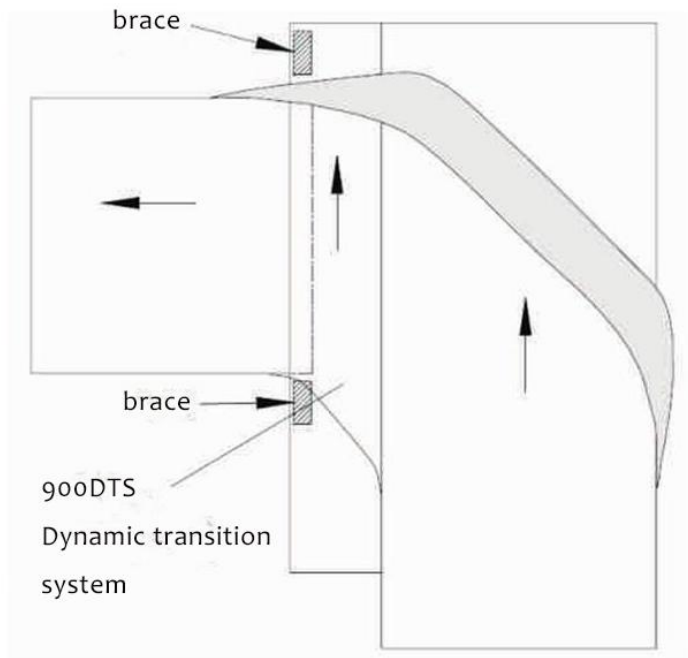
Parabolic guide bar contour with 900DTS dynamic transition system chain.
